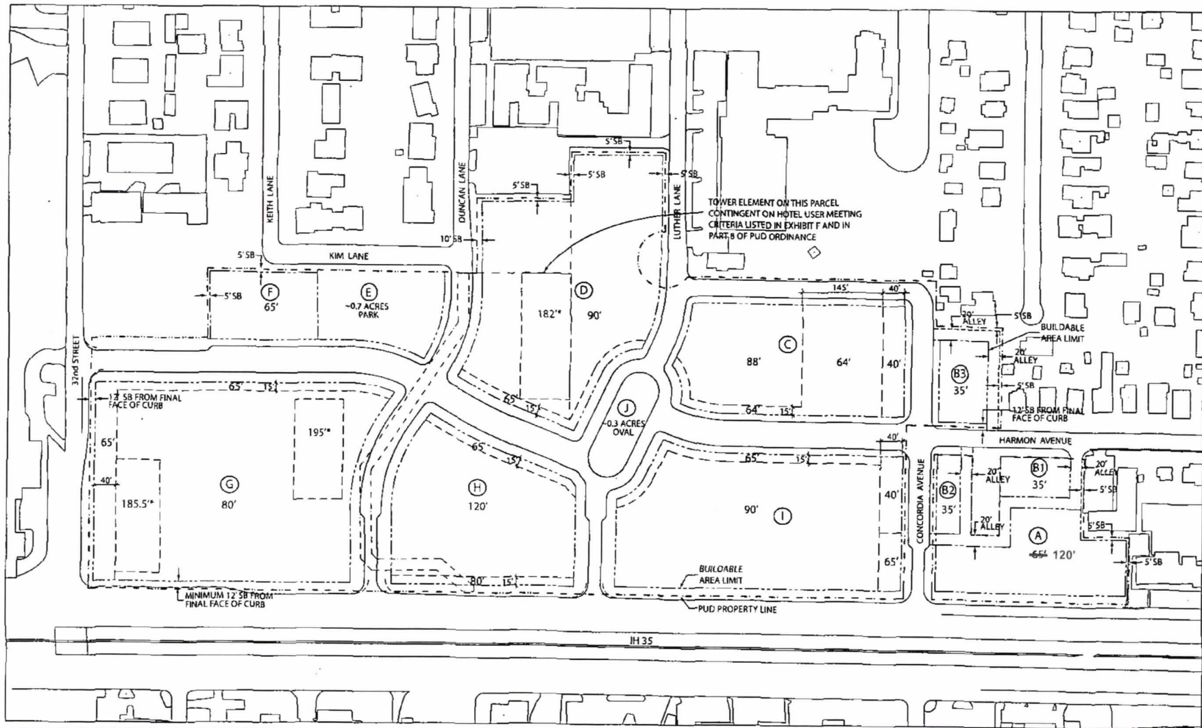
EAST AVENUE PUD EXHIBIT C-2: LAND USE PLAN MAXIMUM BUILDING AREA AND HEIGHT ZONES Prepared by ROMA Design Group
